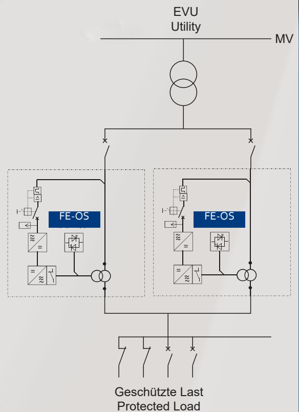
Paralleling of FE-OS systems with equal power rating
